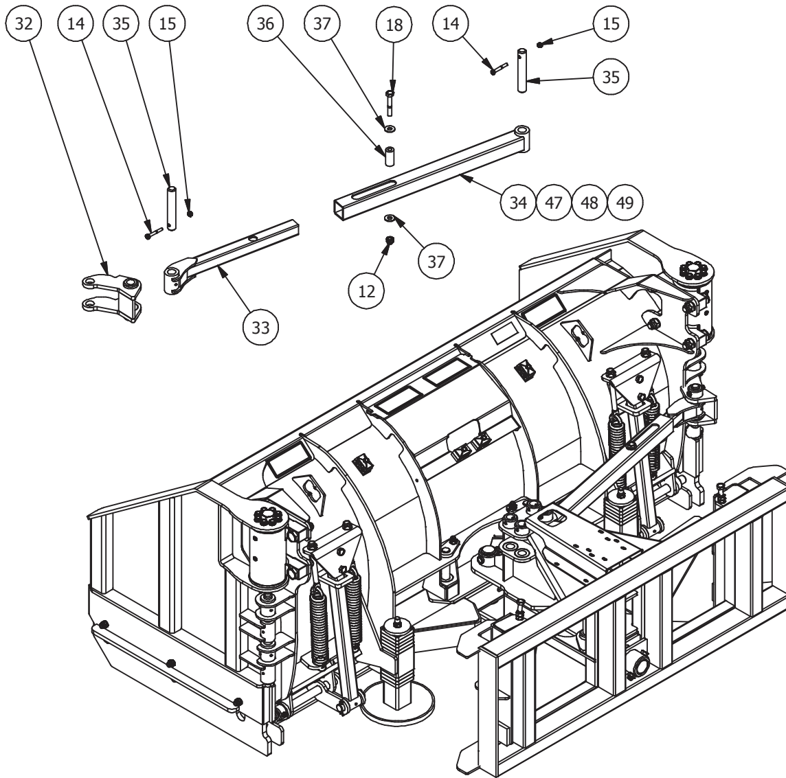
Parts List
